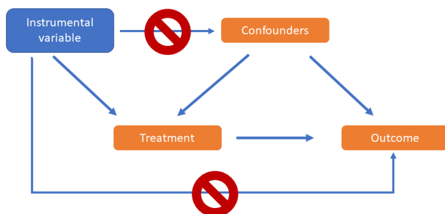
Figure 4.1. Instrumental variable 43
